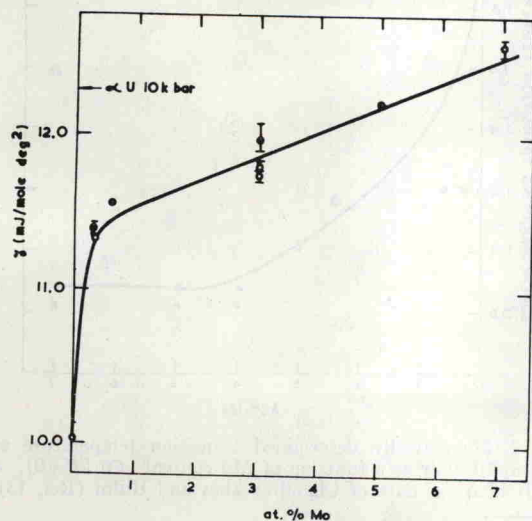
FIG. 4. Coefficient of electronic specific heat \gamma as a function of Mo content.
