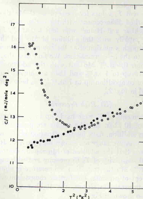
FIG. 5. Heat-capacity data for the 0.3-at.-% Mo alloy taken in zero field and 8 kG: \circ ( H=0 ), \bullet ( H=8 ) kG.
